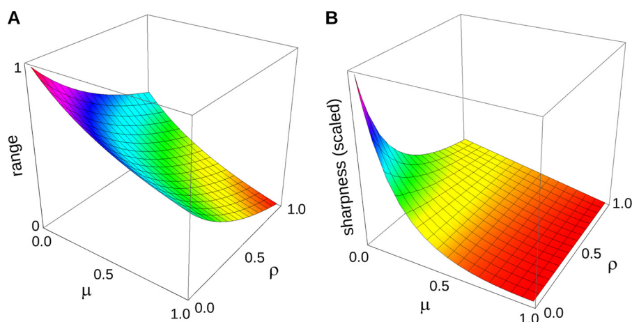
FIGURE 2. Range and sharpness are maximized when both enzymes are perfectly irreversible. A, range of u_1 given by Equation 5 is plotted as a function of the relative catalytic efficiencies, \mu and \rho . The enzymes are assumed to be biased in their normal directions, so that 0 < \mu, \rho < 1 , as shown, with 0 being perfect irreversibility. The maximum range is attained when both enzymes are perfectly irreversible. B, sharpness of switching given by Equation 7 is plotted as a function of the relative catalytic efficiencies, \mu and \rho , with the relative binding affinities set to \alpha = \beta = 0.1 . The units on the vertical axis are omitted, as Equation 7 shows that the sharpness can be rescaled by \phi , which reflects the relative strength of the two enzymes. As long as the enzymes are biased in their normal directions, with 0 < \mu, \rho < 1 as shown, maximum sharpness is attained when both enzymes are perfectly irreversible. A proof is given in the "Appendix."
